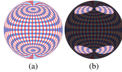
Figure 3. Polarization reversal. A synthetic rendering (a) of a pattern of blue lines of latitude and red lines of longitude reflected on a mirror ball exhibits regions where the horizontal and vertical axes appear exchanged (highlighted in (b)).
