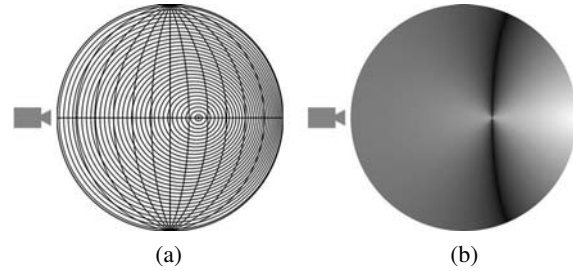
Figure 4: (a) Hemispherical angular map representation of directions of linear polarization for independent specular and subsurface reflection for a full sphere of illumination. The full sphere is derived by mirroring this hemisphere. The camera is assumed to lie to the left. (b) Attenuation of specular reflection, represented in the same space as (a). Near the Brewster angle the reflection is weak, making recovery of true specular reflectance unstable.
